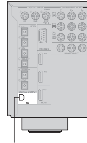
XM jack
