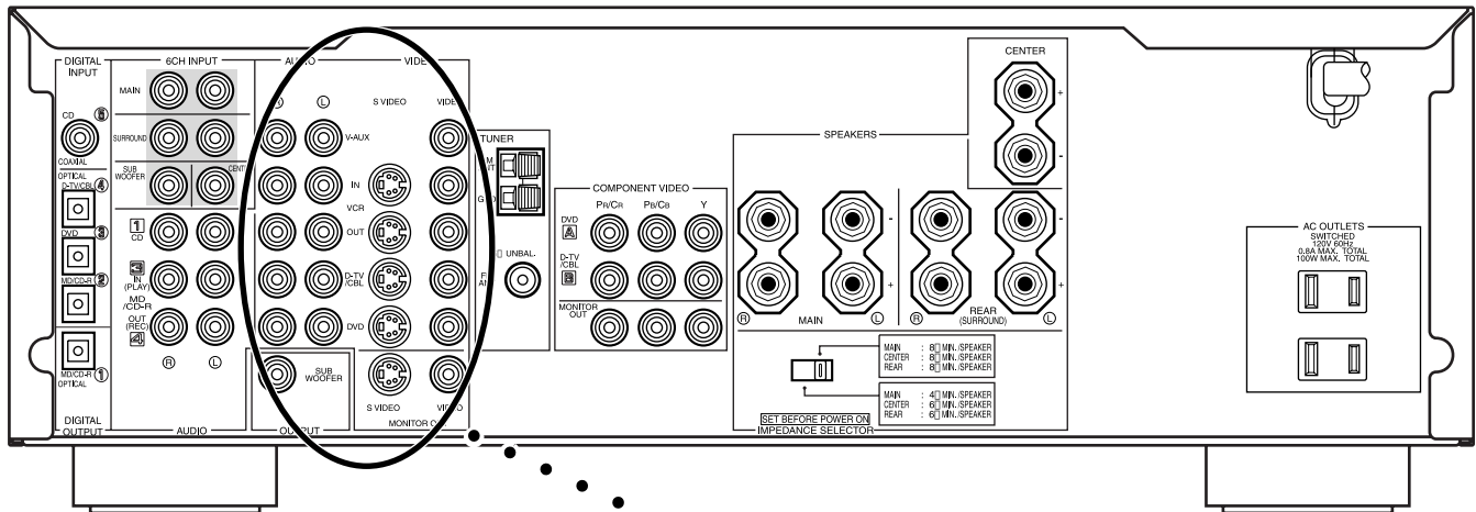
Yamaha HTR-5550 Receiver (Rear Panel)
